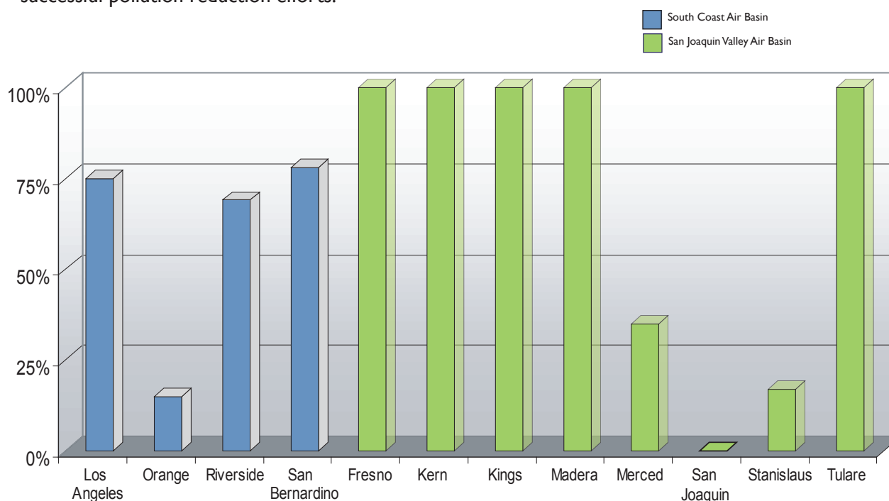
Figure E-1. Percent of the population exposed to PM 2.5 concentrations above the average annual federal standard (15 µg/m 3 ) in 2005-2007 by county.
